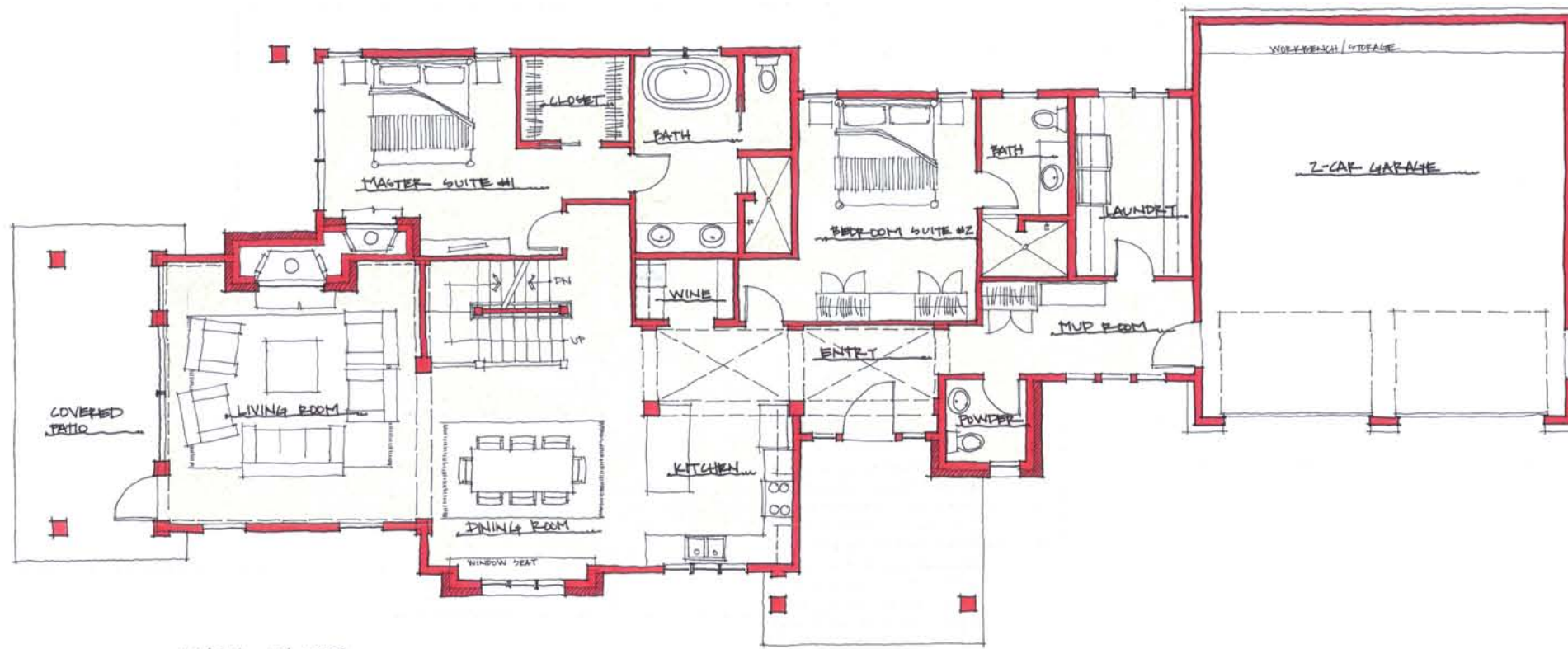
MAIN FLOOR
